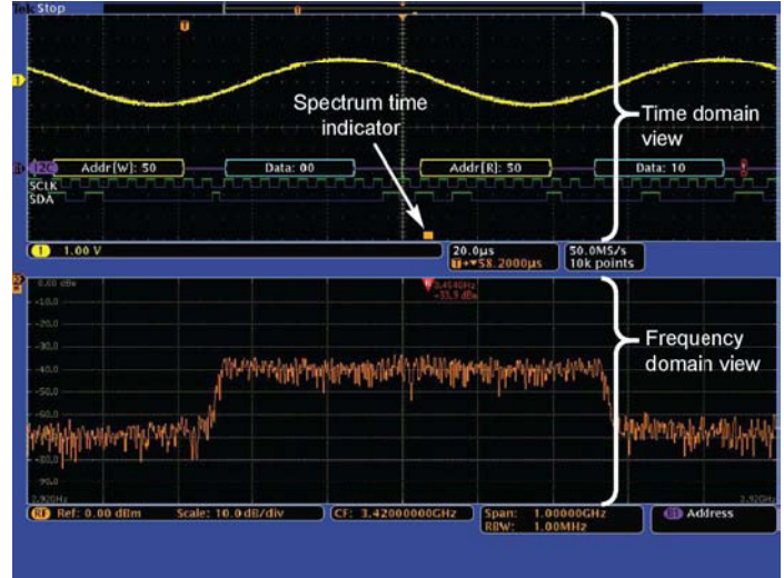
The upper half of the MDO4000 Series display shows the Time Domain view of the analog and digital channels, while the lower half shows the Frequency Domain view of the RF channel. The orange bar - Spectrum Time - shows the period of time used to calculate the RF spectrum.
