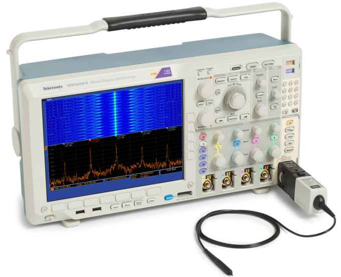
The optional TPA-N-VPI adapter enables any active, 50 Ω TekVPI probe to be connected to the RF input.
