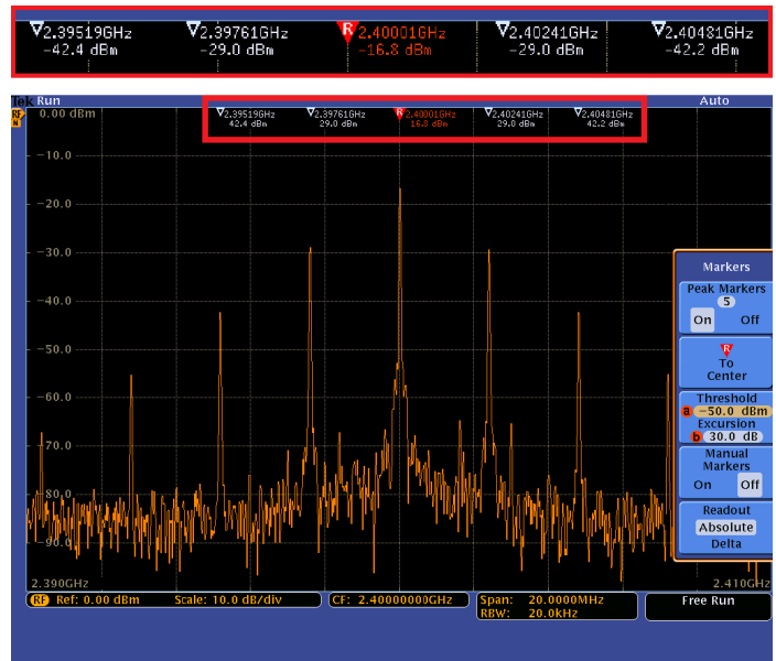
Automated peak markers identify critical information at a glance. As shown here, the five highest amplitude peaks that meet the threshold and excursion criteria are automatically marked along with the peak's frequency and amplitude.
